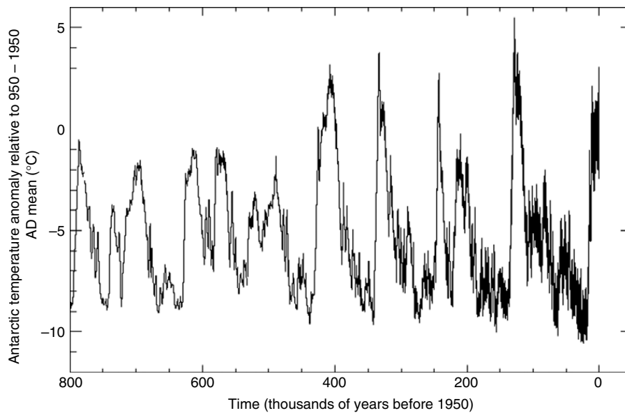
Fig. 1. 800,000-year record of Antarctic temperature change.
