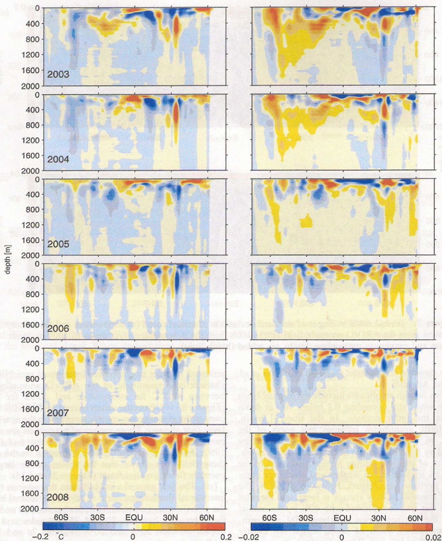
Figure 8. Yearly zonal average of (left) temperature and (right) salinity anomalies in the Pacific basin during 2003–2008 for the upper 2000 m depth.
