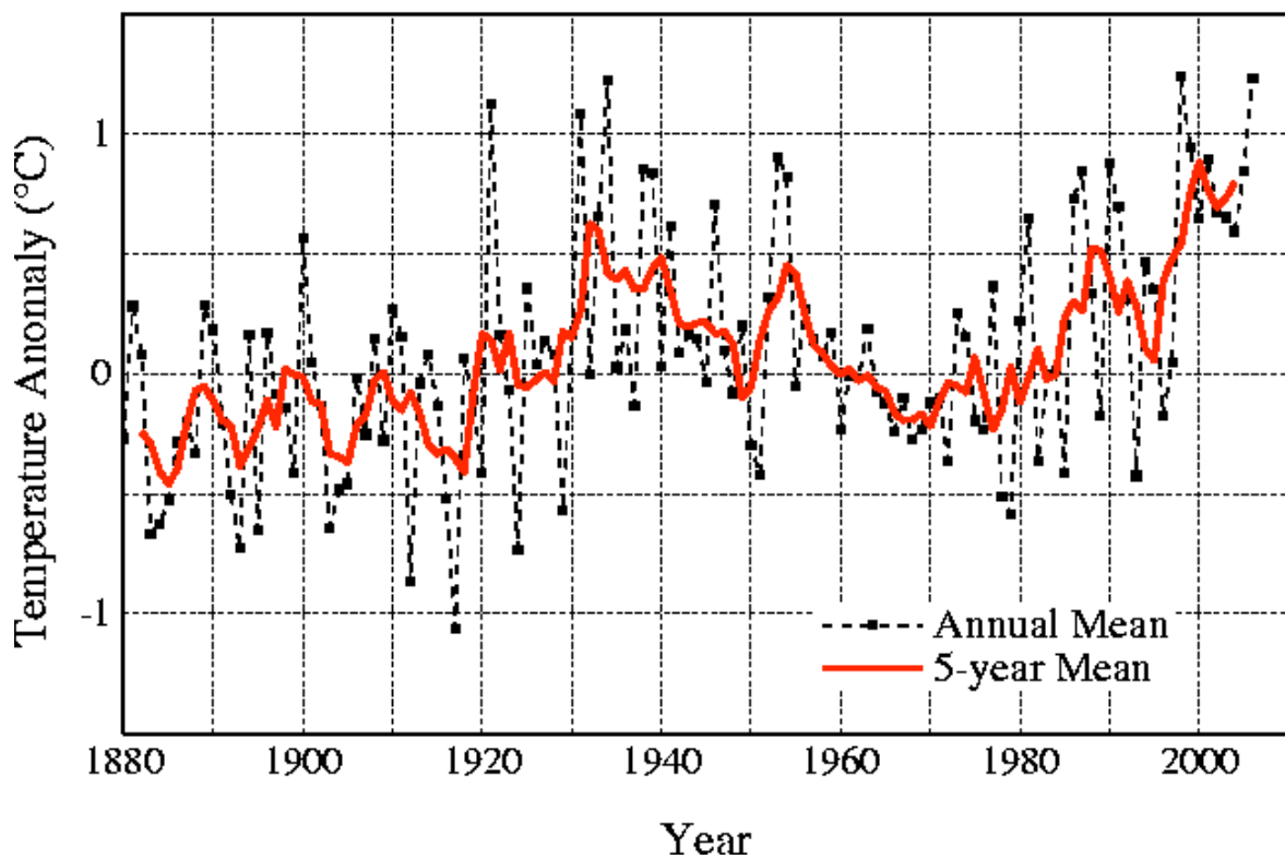
Figure 3 United States temperature anomaly record (Hansen, Goddard Institute of Space Studies, 2007) ..
