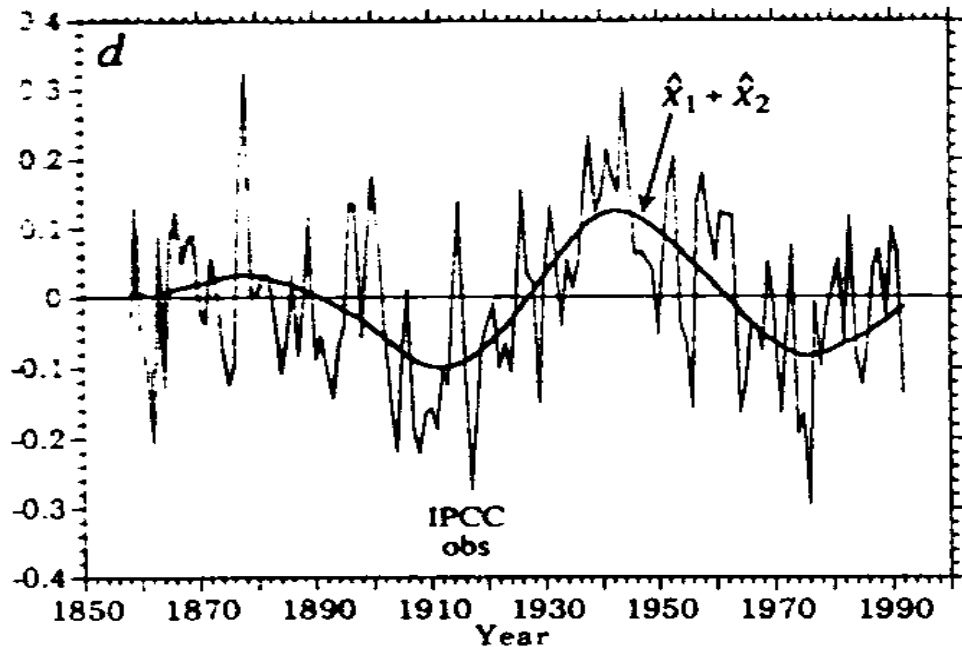
Figure 5. Global temperature oscillation identified by Schlesinger and Ramankutty 1994
