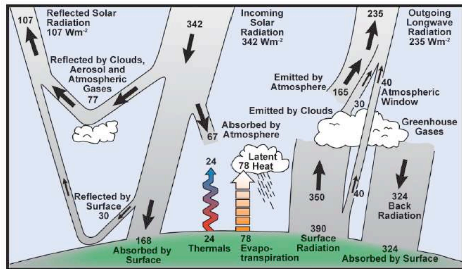
Figure 1 Earth’s Annual Global Mean Energy Budget, as envisaged by Kiehl and Trenberth (1997)
