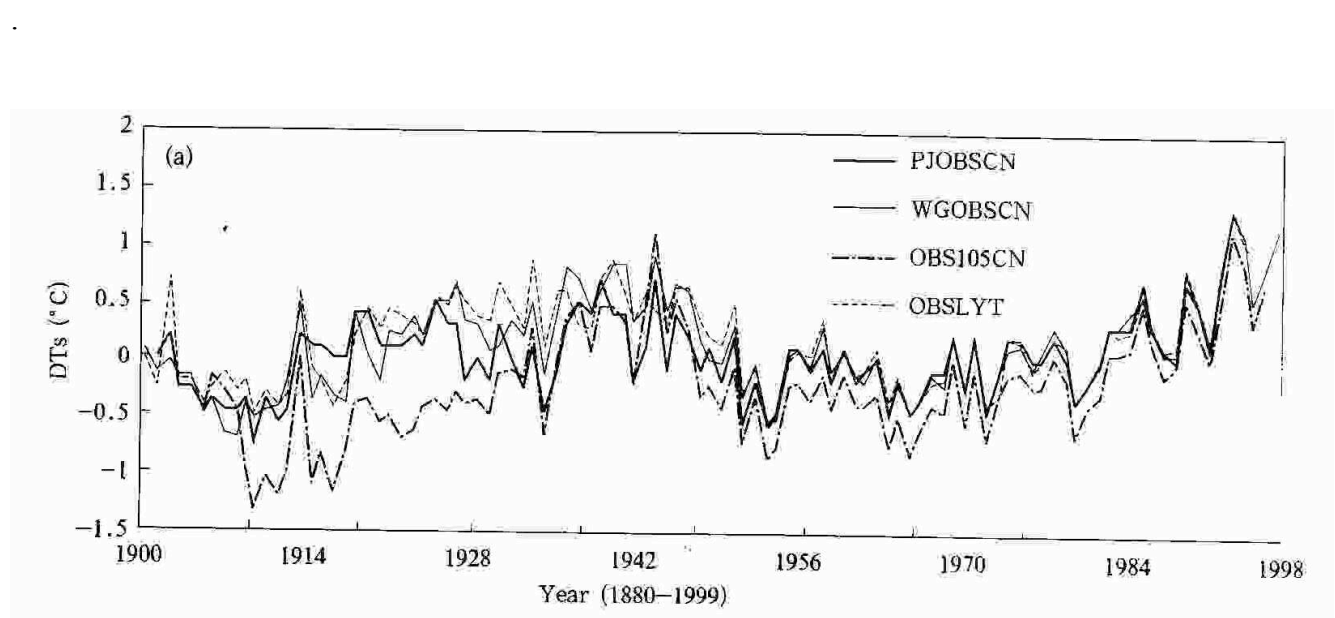
Figure 7. Temperature anomaly record for China (Zhao et al 2005). Black curve from Jones (personal communication) the other curves from different Chinese investigators.
