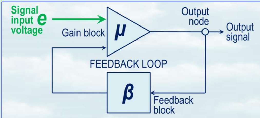
Fig. 4 Feedback-amplifier block diagram (Black 1934). The input signal e is the no-greenhouse-gas emission temperature climate scientists had overlooked.
