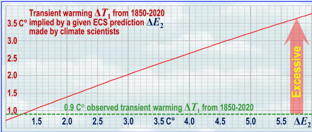
Fig. 12 All current predictions of final warming (ECS) of 2^\circ\text{C} or more by doubled \text{CO}_2 imply warming from 1850-2020 far above the observed 0.9^\circ\text{C} .
