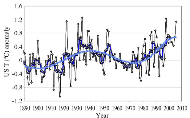
Figure 6. US average temperature anomaly with GCDC 2007 correction, with a wavy pattern but with lower rising trend (NOAA) [15].
