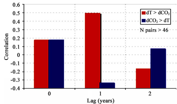
Figure 9. Correlation between interannual changes in CO 2 (ppmv) at Mauna Loa and in temperature (°C) at tropical band, north hemisphere). Low, positive correlation for the same year; strong correlation for temperature leading CO 2 changes in the following year.
